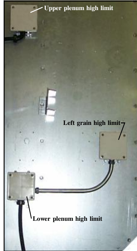
Grain temperature thermister. There are 2 thermisters in each (right & left) grain high limit thermostat assemblies.
